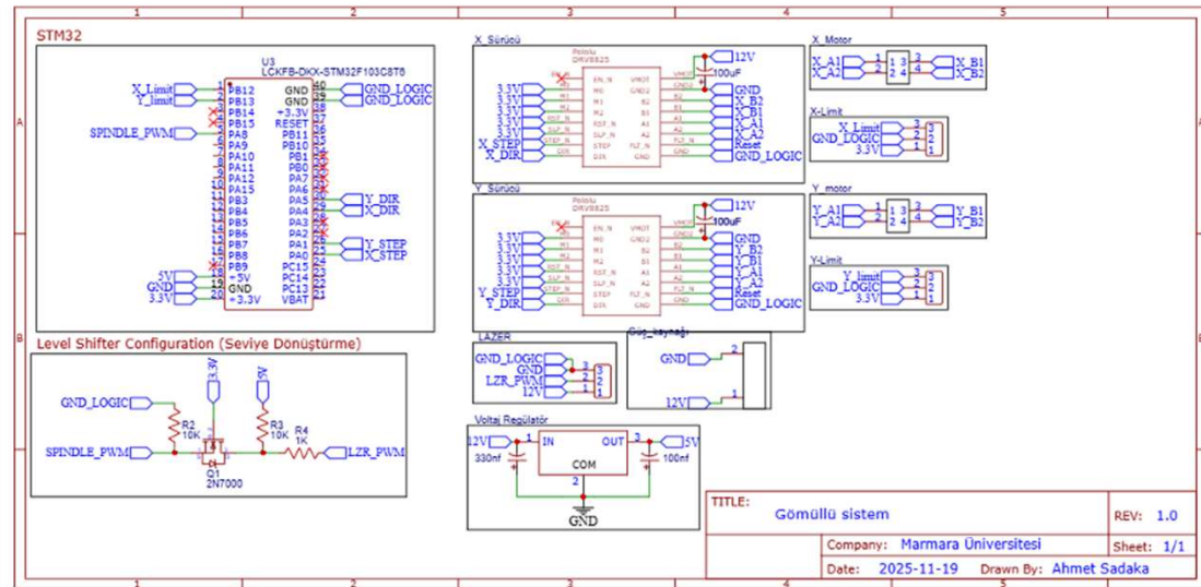
System wiring diagram
